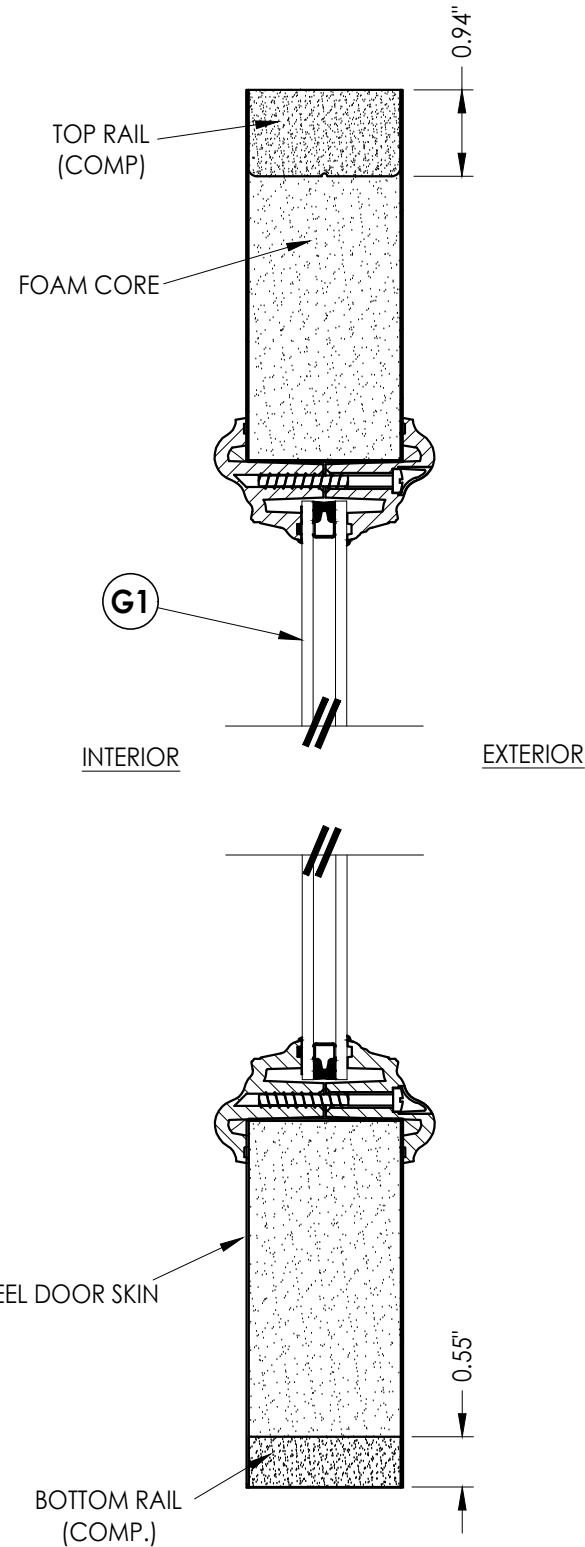
2 4 VERTICAL CROSS SECTION
